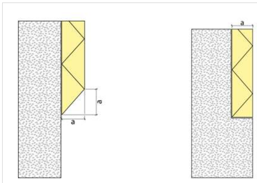
Figuur 315.2 - Detaillering hittewerende bekleding
